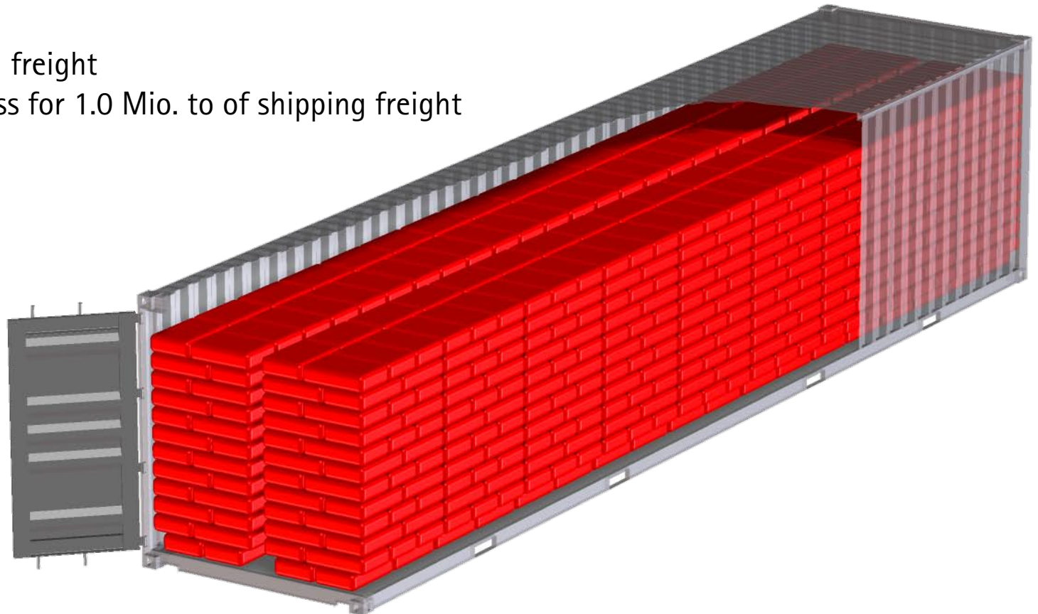
FEU with 18 (2x9) packages each 1,475 kg
